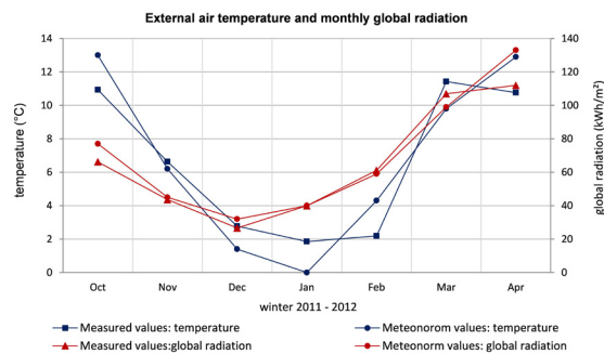
Fig. 51: Comparison of measured monthly average temperatures and monthly sum of horizontal global radiation with Meteorological climate data.
