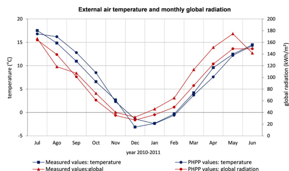
Fig. 83: Comparison with standard weather data from PHPP
