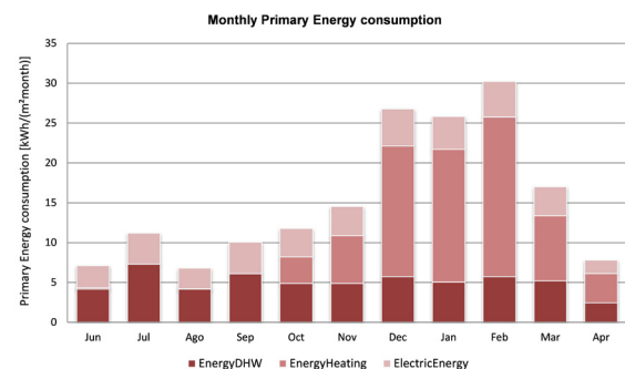
Fig. 84: Monthly primary energy consumption
