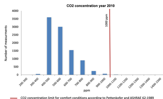
Fig. 93: CO 2 measurements distributed by steps of 100ppm in ambient 1.
