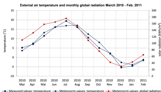
Fig. 65: Comparison of measured monthly average temperatures and monthly sum of horizontal global radiation with Meteonorm climate data.
