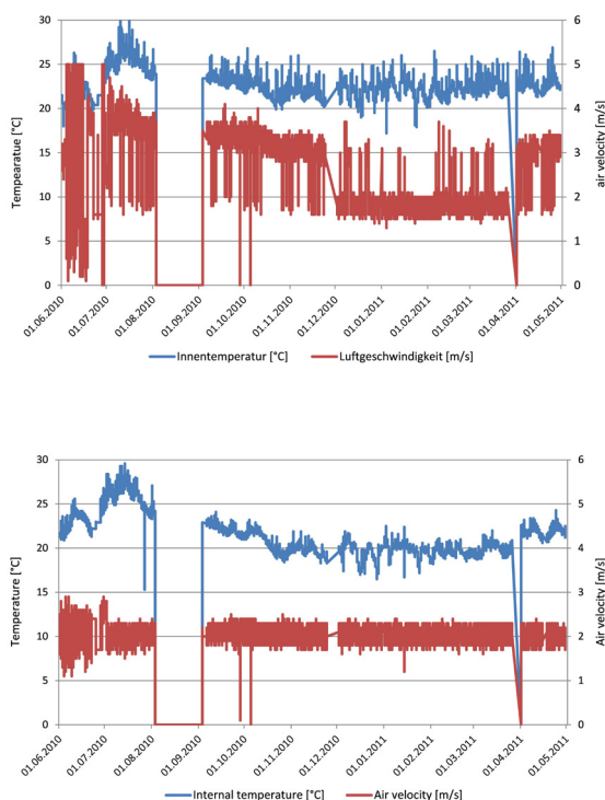
Fig. 108 and 109: Comparison of air velocity in supply air duct of two different flats
