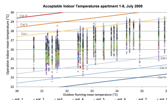
Fig. 49: Evaluation of thermal comfort in summertime for eight apartments in a multifamily building.
