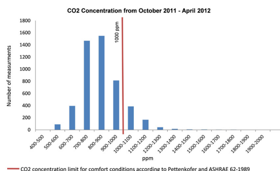
Fig. 57: CO 2 concentrations during the heating period.
